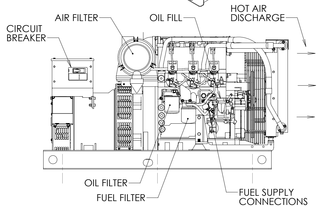
SERVICE SIDE
